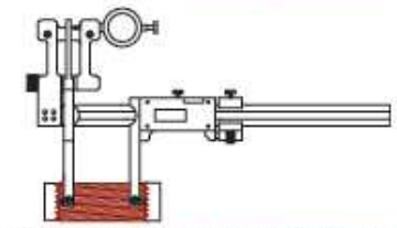
Controllo filettature interne Inside thread measurement
