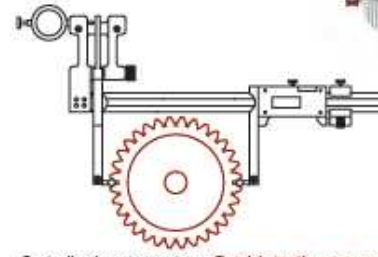
Controllo dentature esterne Outside tooth measurement
