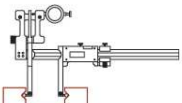
Controllo canali e gole interne Inside channel and groove measurement
