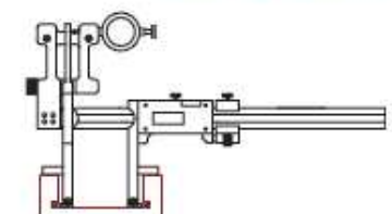
Controllo canali e gole interne Inside channel and groove measurement
