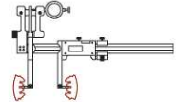
Controllo dentature interne Inside tooth measurement
