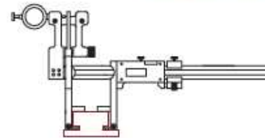
Controllo canali e gole esterne Outside channel and groove measurement
