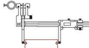
Controllo canali e gole esterne Outside channel and groove measurement
